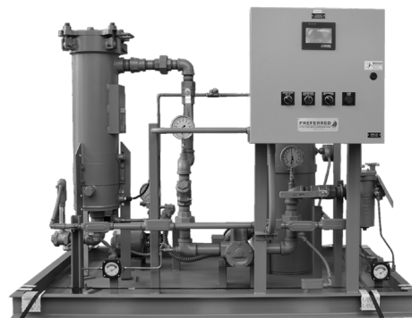
Picture with WR 3I Chem Injection Version
